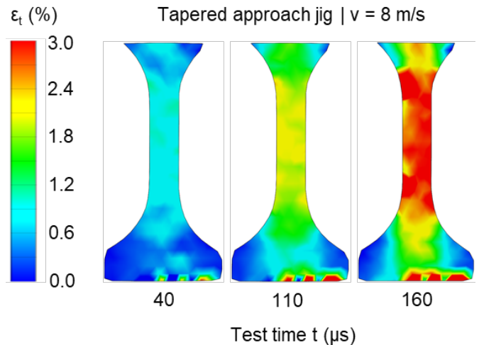
Figure 7: Specimen strain distribution at diff. test times
